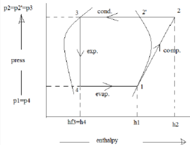
Fig. 14. P-h diagram for Dry Vapour Compression Cycle
