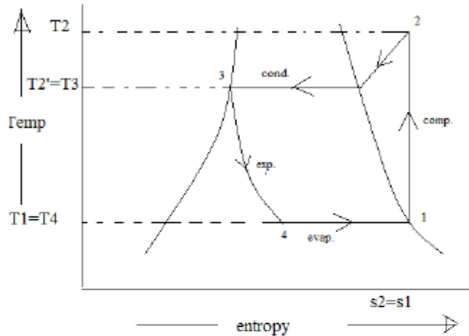
Fig.13 T-S diagram for Dry Vapour Compression Cycle
