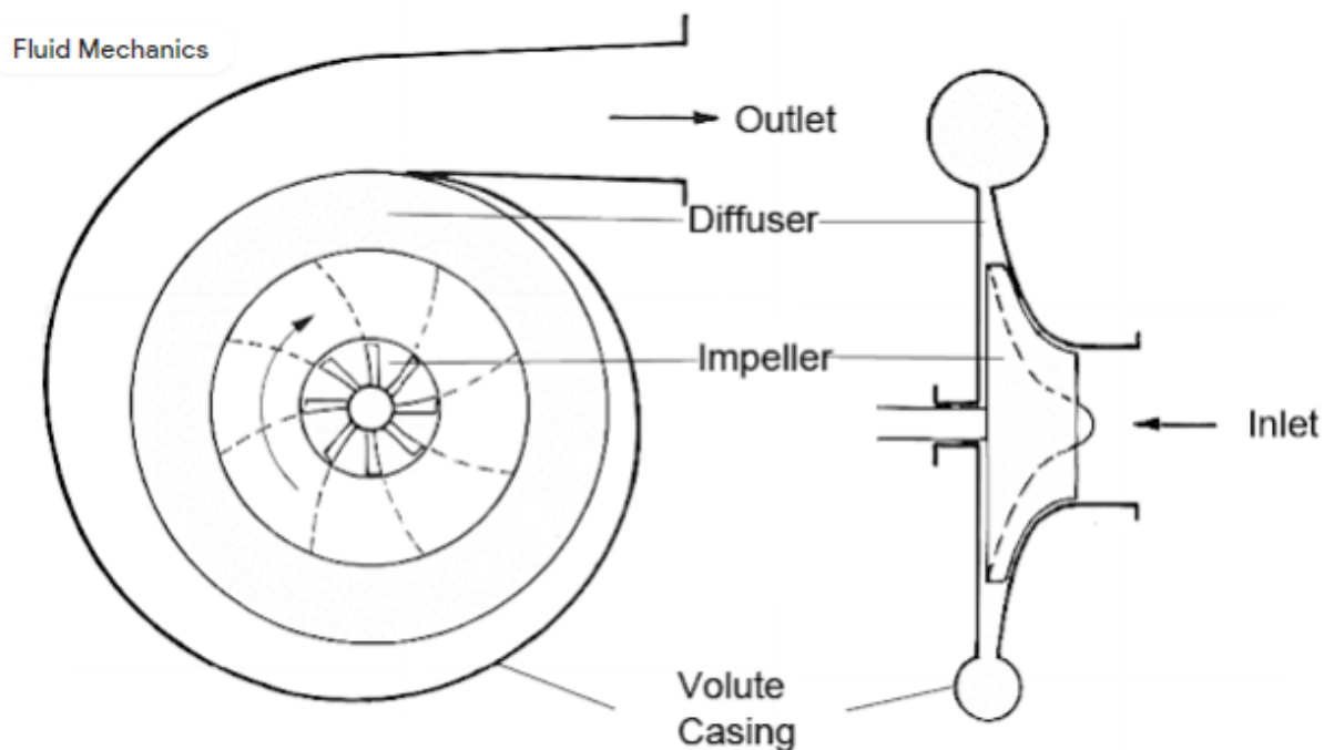
Centrifugal compressor schematic diagram
