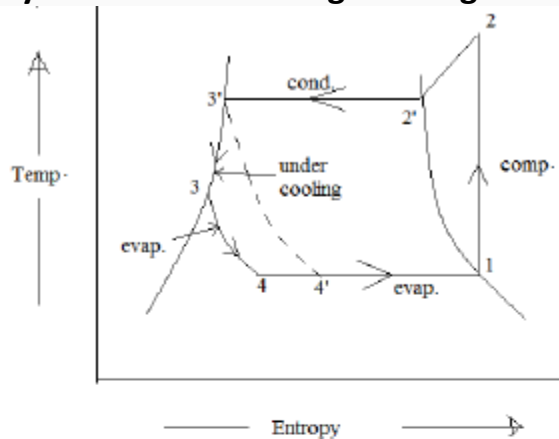
17. T-S diagram for Vapour Compression cycle with undercooling refrigerant.
