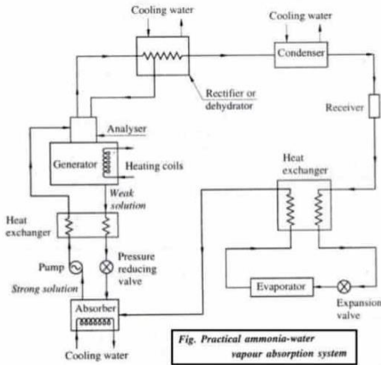
practical ammonia -water vapour absorption system
