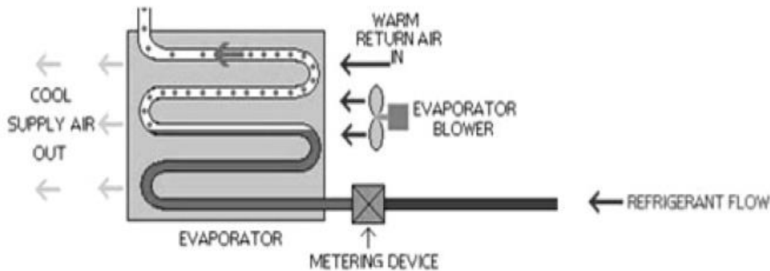
Figure: Evaporator
