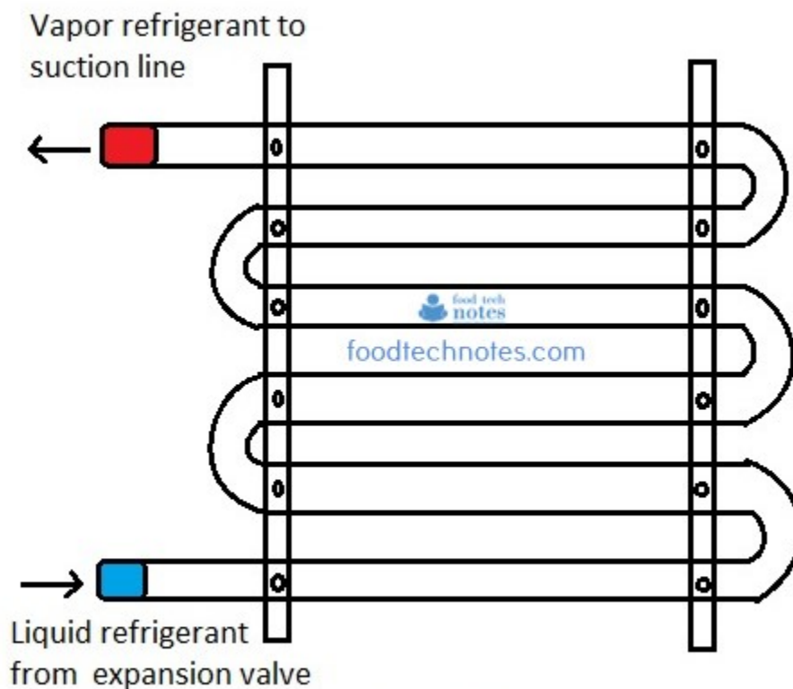
Fig: Bare tube evaporator
