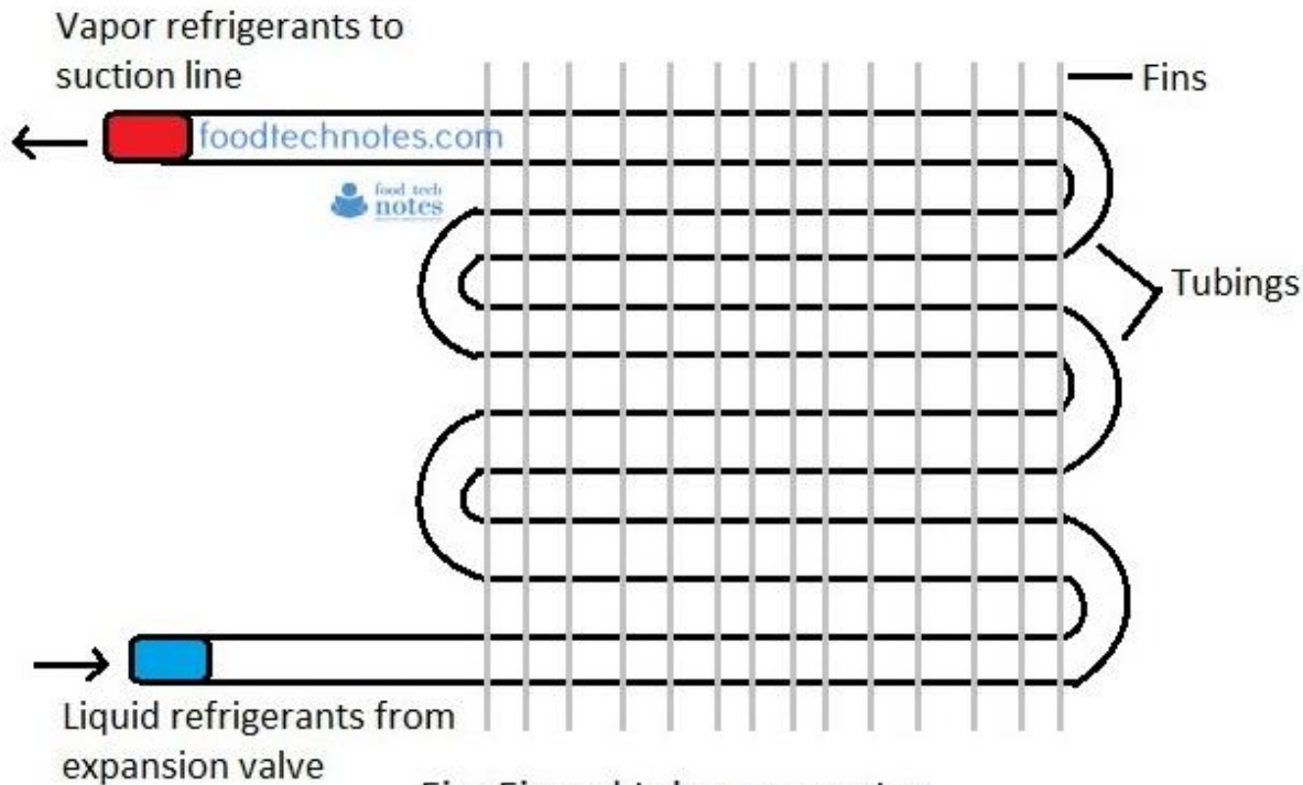
Fig: Finned tube evaporator
